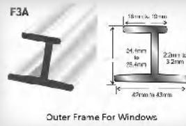
F-PROFILE
